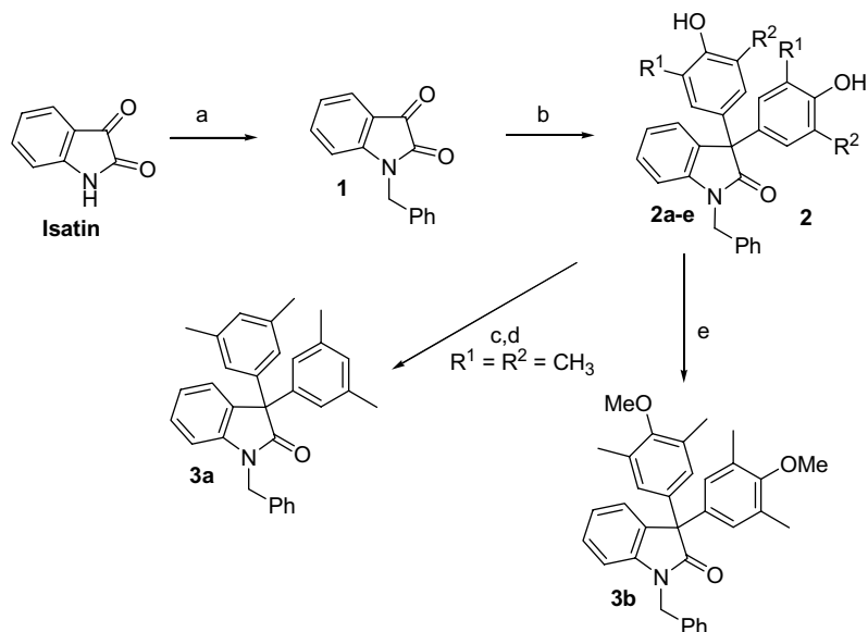
Scheme 1. Reagents and conditions: (a) KO- t -Bu, BrBn, 84%; (b) excess phenol, TfOH, 50–70%; (c) 2,4,6-collidine, Tf 2 O, 67%; (d) n -Bu 3 N, Ph 2 P(CH 2 ) 3 PPh 2 , PdCl 2 (PPh 3 ) 2 , HCO 2 H, DMF, 58%; (e) Cs 2 CO 3 , MeI, DMF, 40 °C, 76%.
