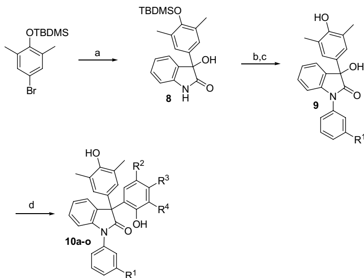
Scheme 3. Reagents and conditions: (a) n -BuLi/THF/−70 °C, then isatin, 80%; (b) R_1\text{PhB(OH)}_2 , \text{Cu(OAc)}_2 , TEA, 4 Å sieves, 64%; (c) TBAF, 86%; (d) TFA, substituted phenol, 61–75%.
