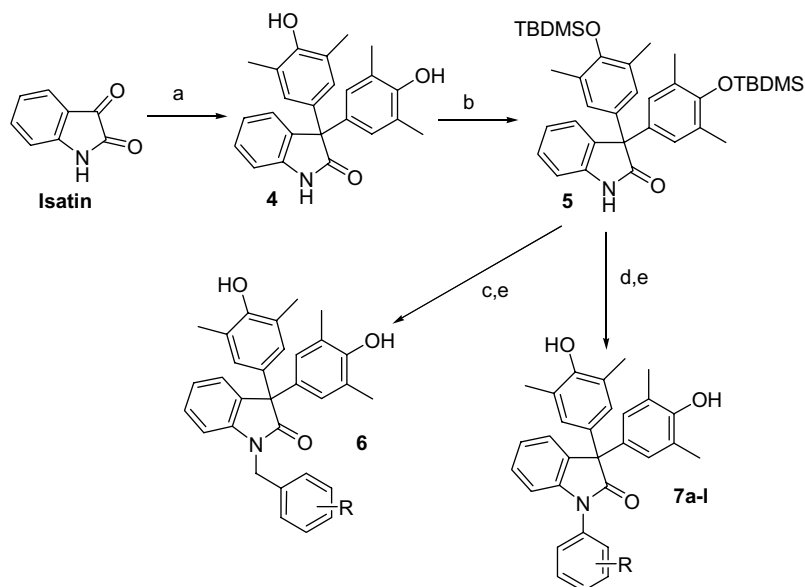
Scheme 2. Reagents and conditions: (a) AcOH, AlCl 3 , 86%; (b) imidazole, DMF, TBDMSCl, 75%; (c) KO- t -Bu, XCH 2 R, 51–66%; (d) RPhB(OH) 2 , Cu(OAc) 2 , TEA, 4 Å sieves, 15–52%; (e) TBAF, 86%.
